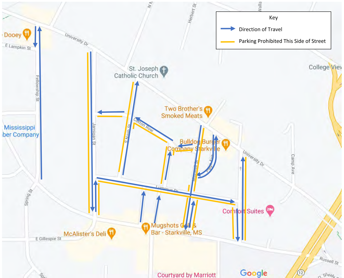
Figure 5.2.3.3 Cotton District Recommended Circulation Improvements
